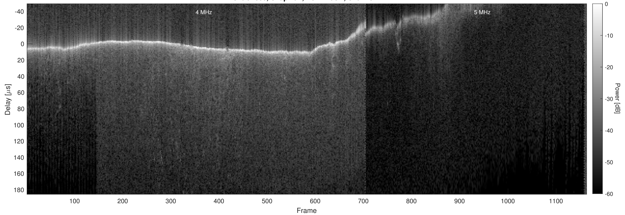
Orbit 7886, Chapman, No Window, Channel 2
