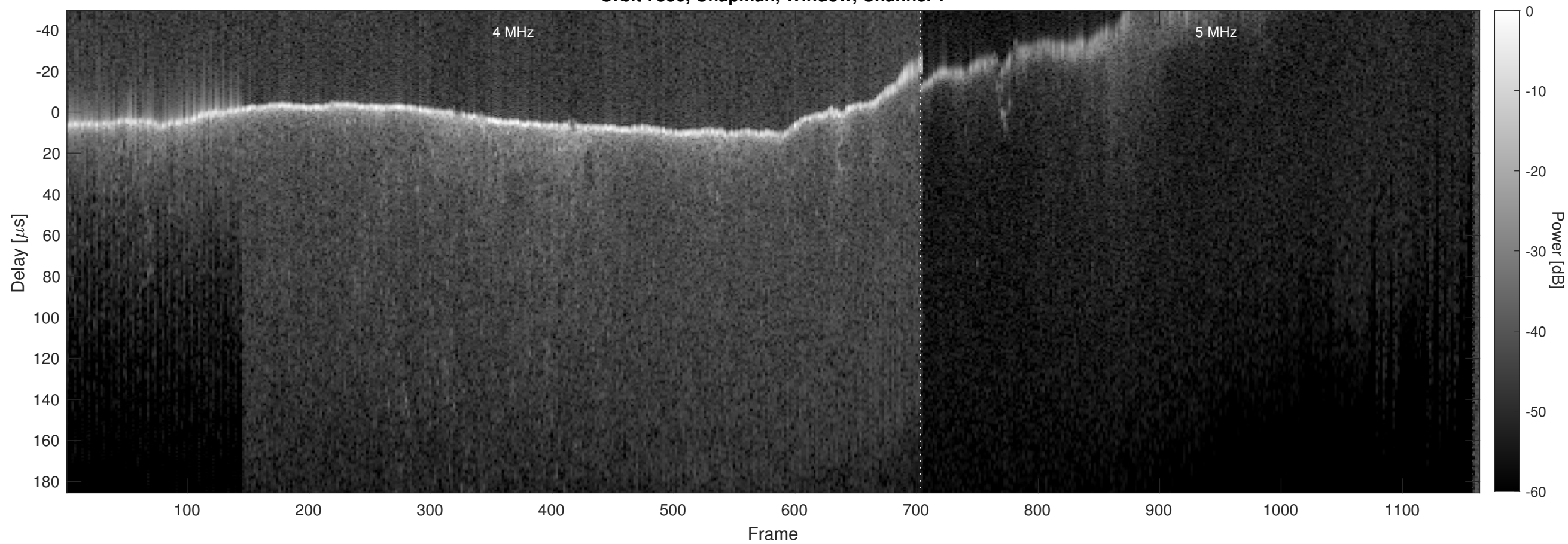
Orbit 7886, Chapman, Window, Channel 2
