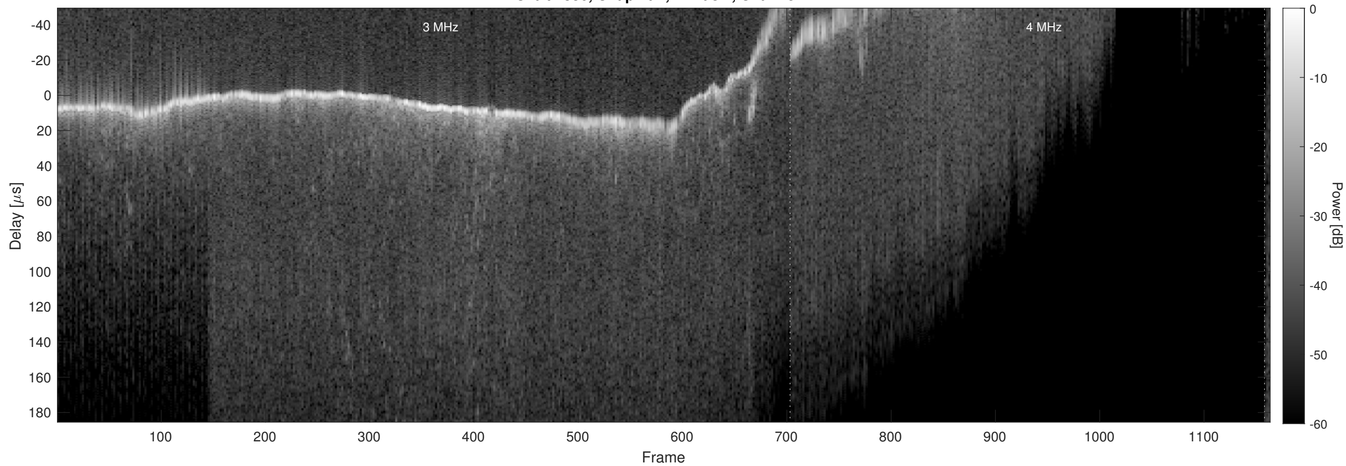
Orbit 7886, Chapman, Window, Channel 2
