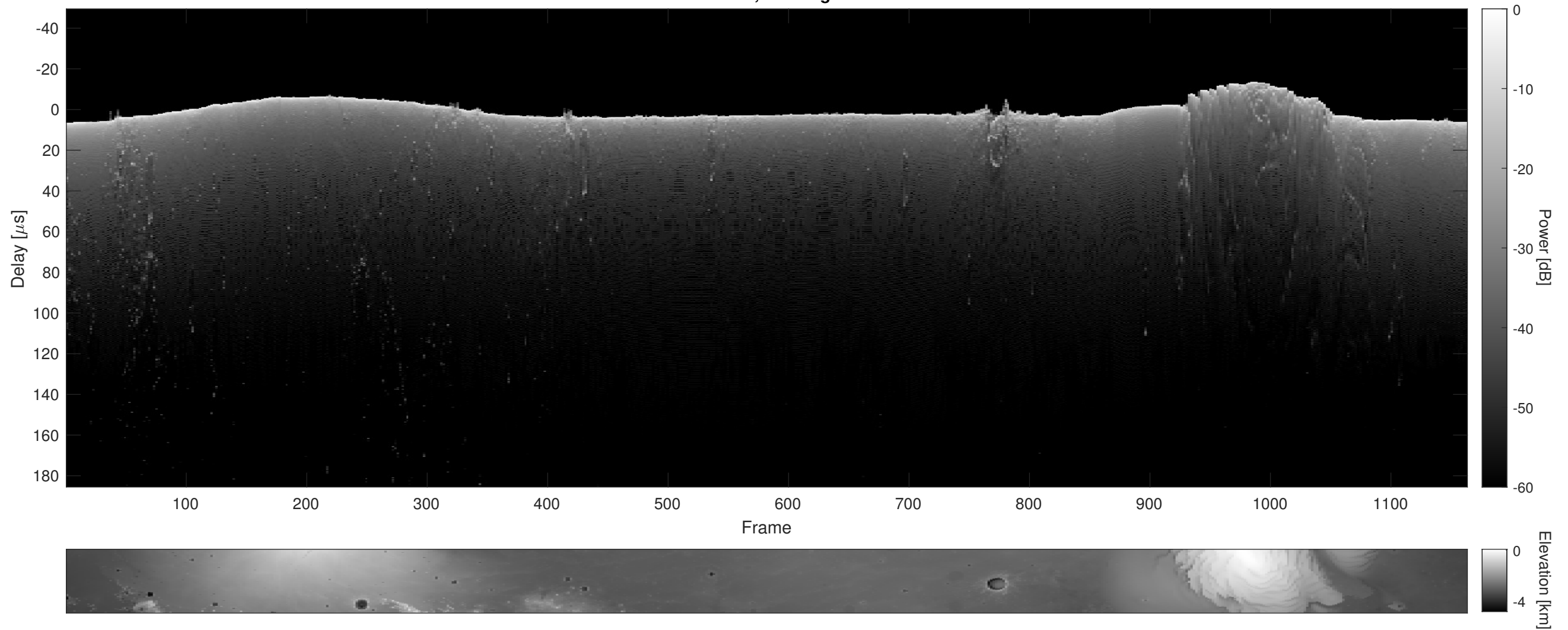
Orbit 7886, Cluttergram
