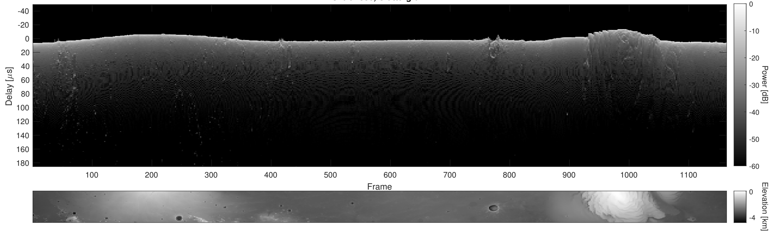
Orbit 7886, Cluttergram
