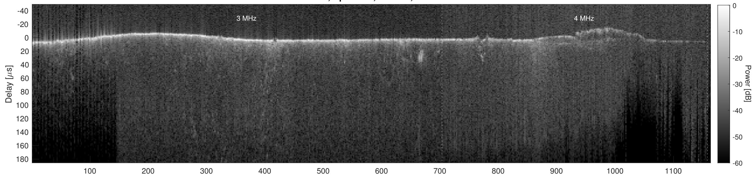
Orbit 7886, Cluttergram
