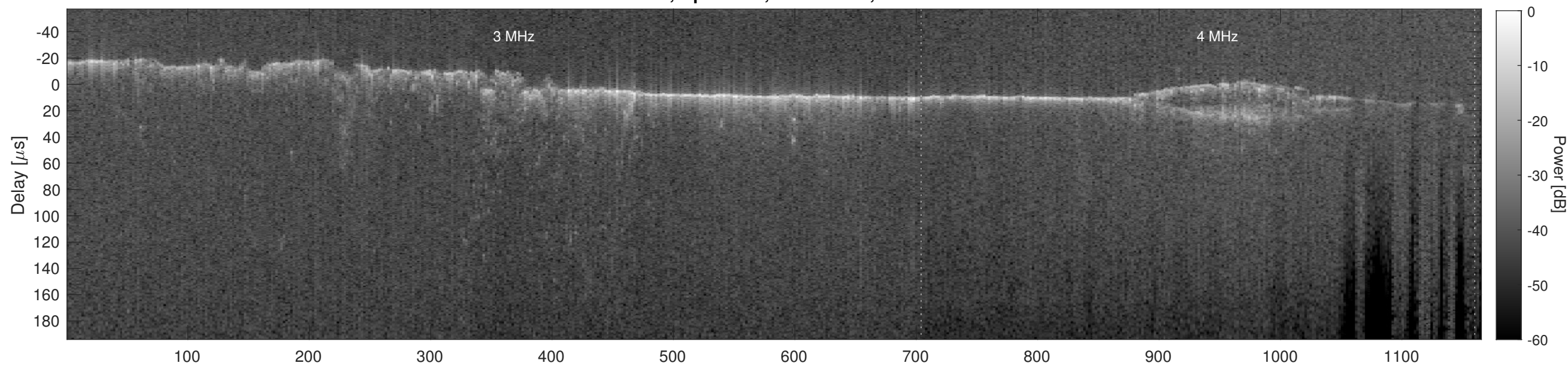
Orbit 7887, Cluttergram
