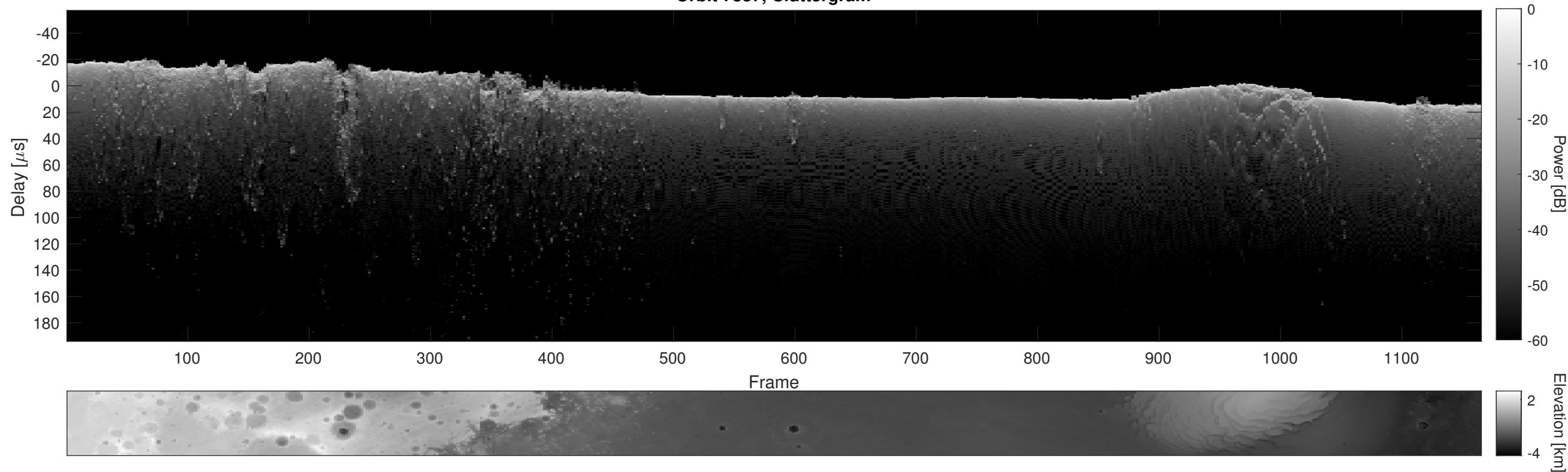
Orbit 7887, Cluttergram
