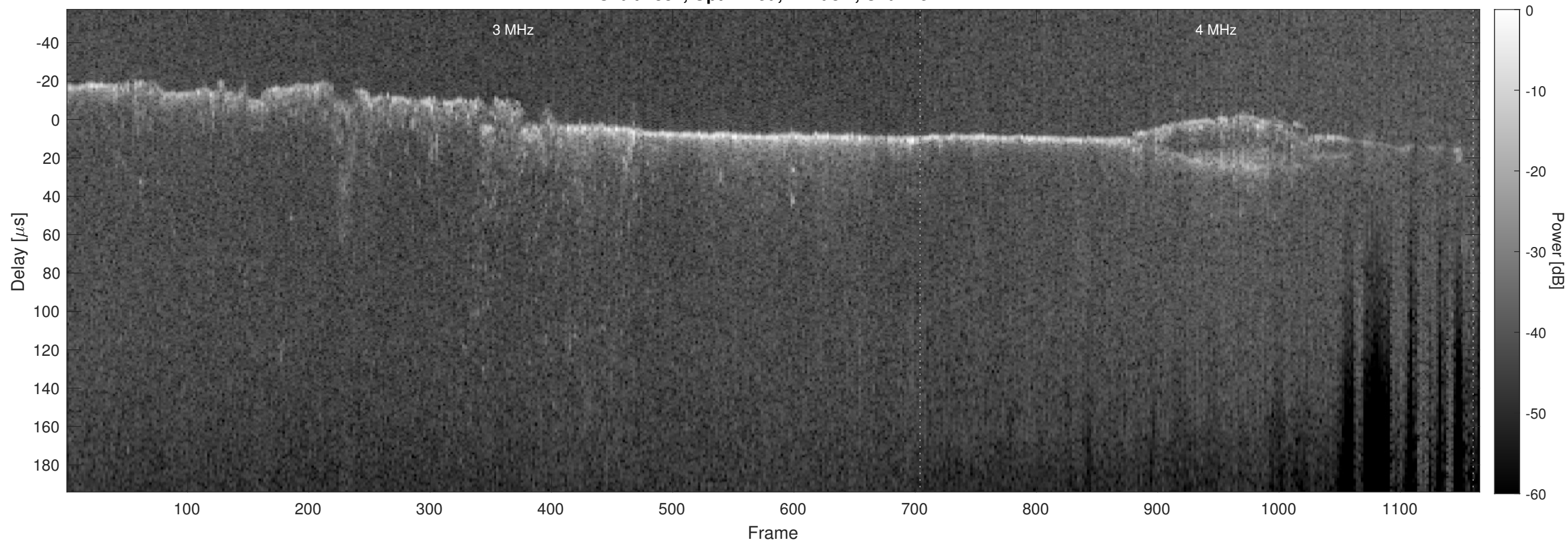
Orbit 7887, Optimized, Window, Channel 2
