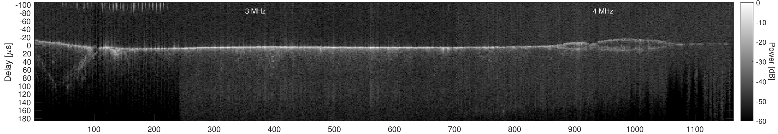
Orbit 7888, Cluttergram
