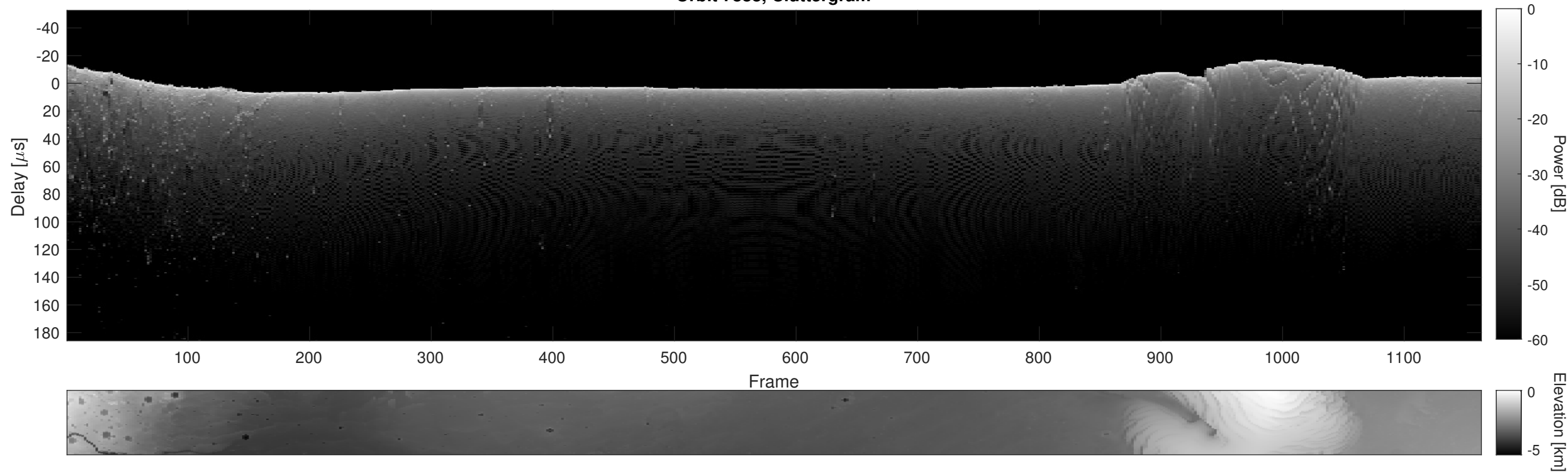
Orbit 7888, Cluttergram
