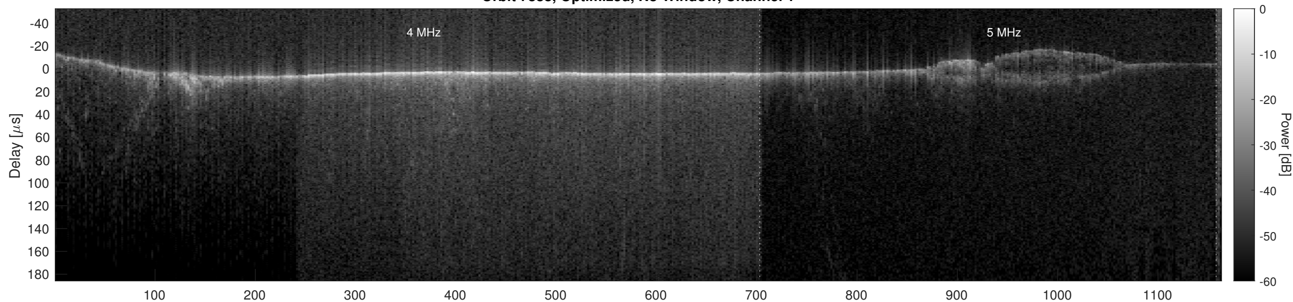
Orbit 7888, Optimized, No Window, Channel 2
