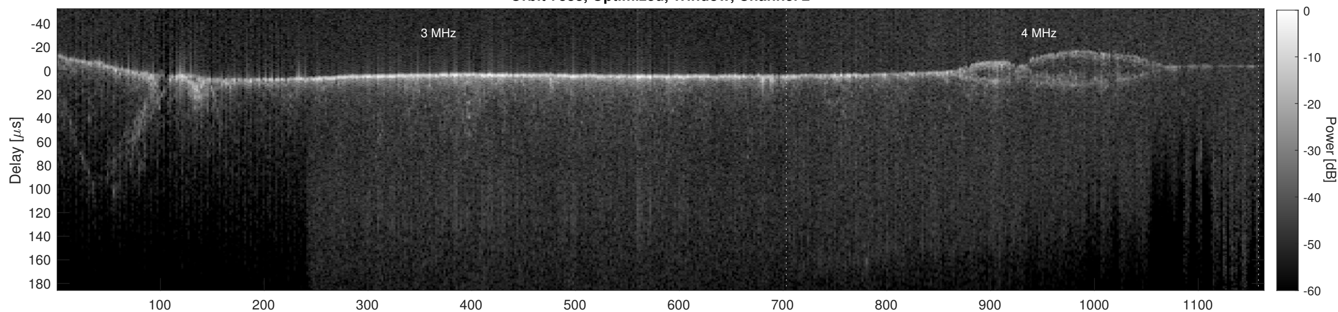
Orbit 7888, Cluttergram
