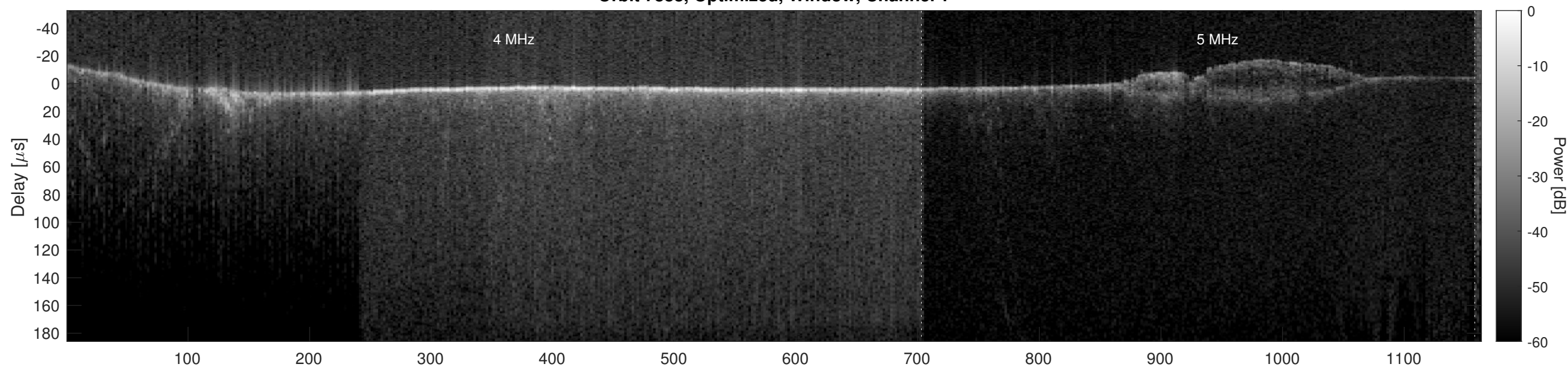
Orbit 7888, Optimized, Window, Channel 2
