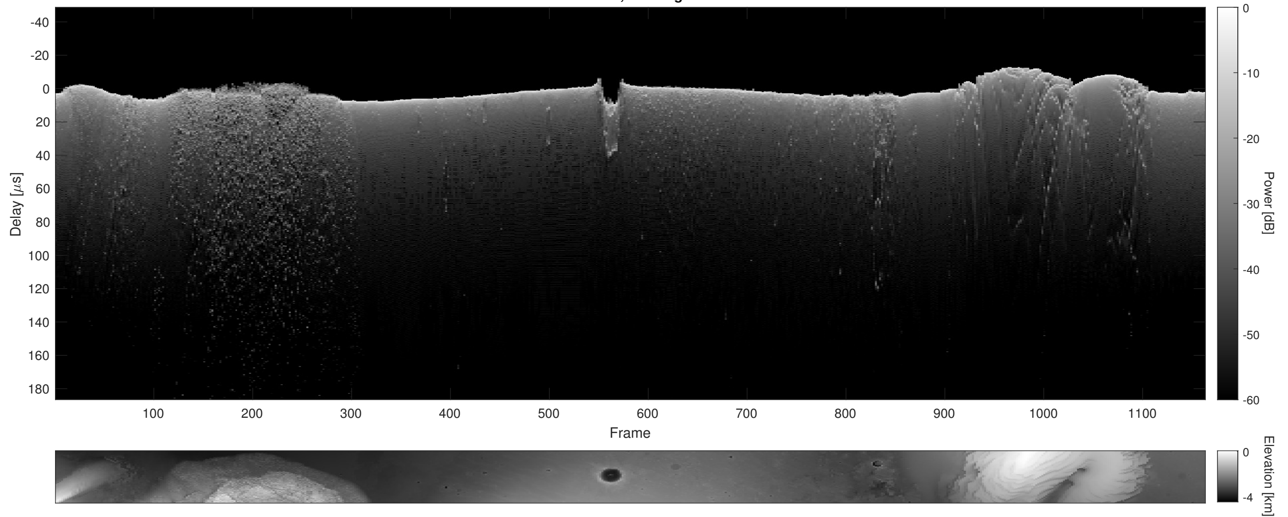
Orbit 7889, Cluttergram
