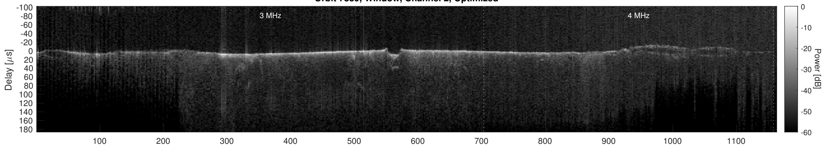
Orbit 7889, Cluttergram
