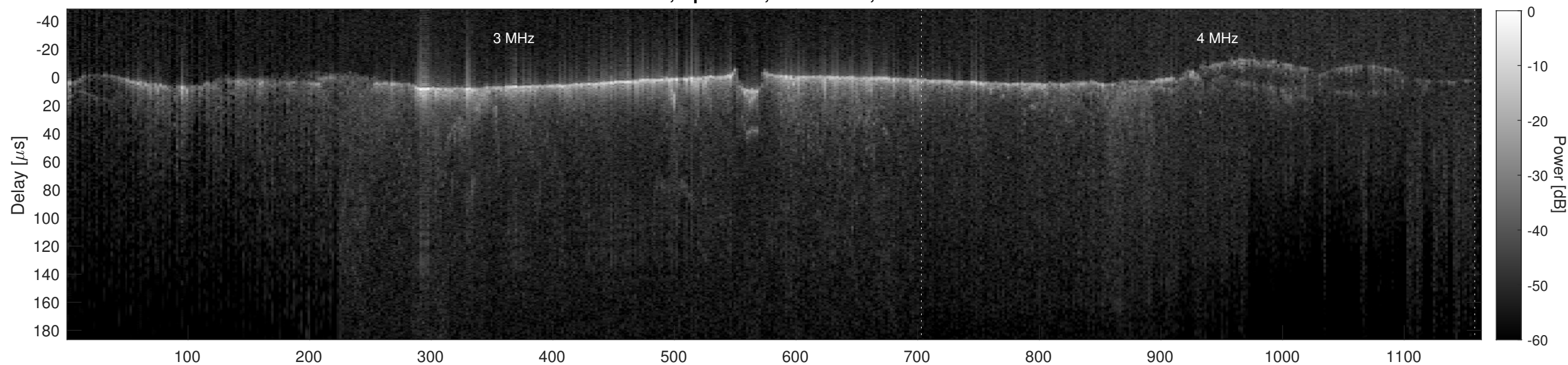
Orbit 7889, Cluttergram
