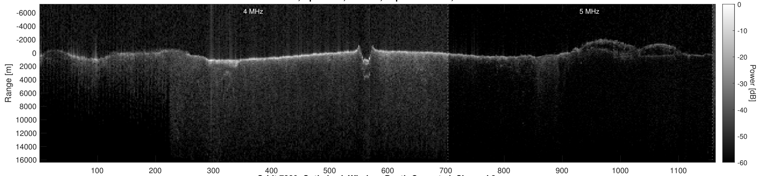
Orbit 7889, Optimized, Window, Depth-Corrected, Channel 2
