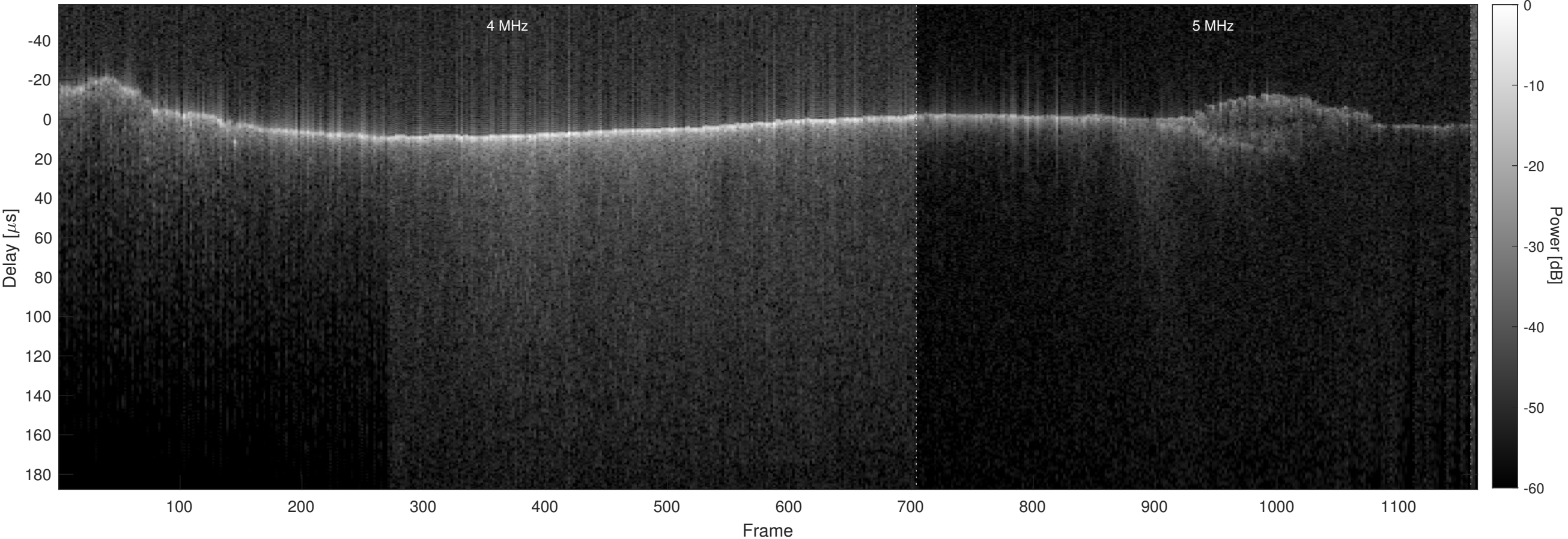
Orbit 7890, Optimized, No Window, Channel 2
