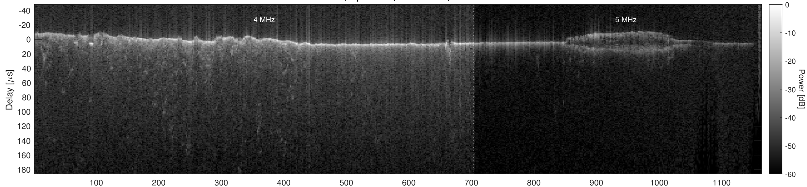
Orbit 7891, Optimized, No Window, Channel 2
