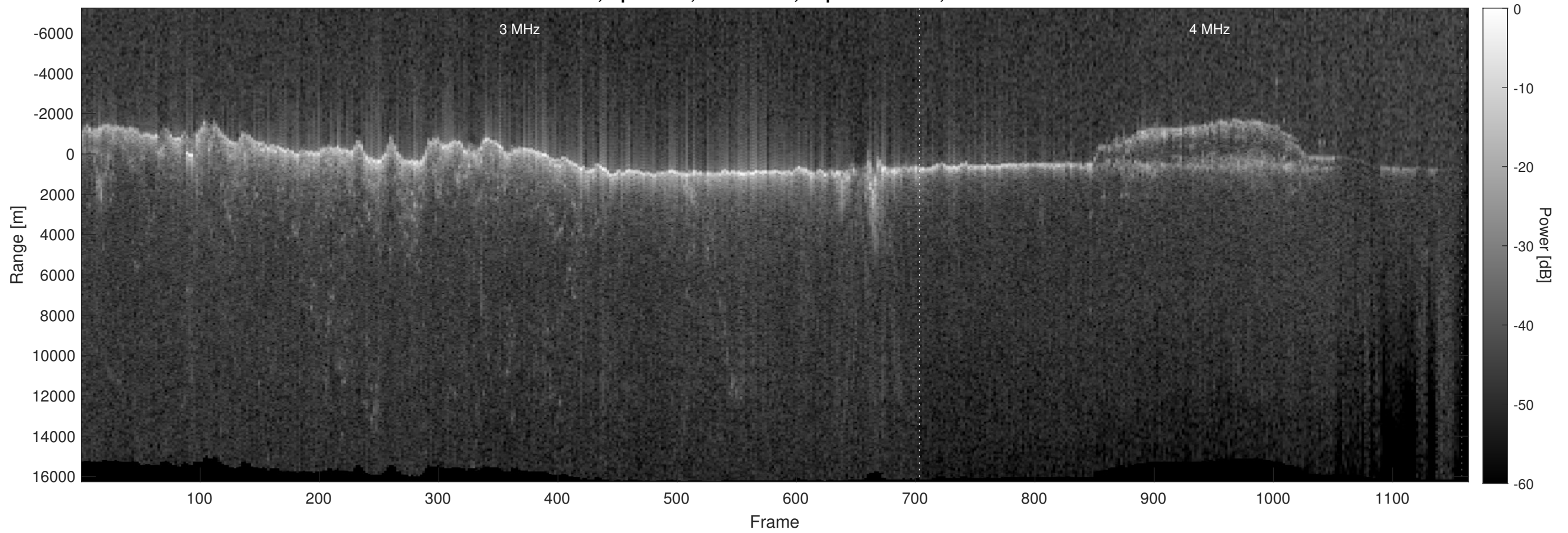
Orbit 7891, Optimized, No Window, Depth-Corrected, Channel 2
