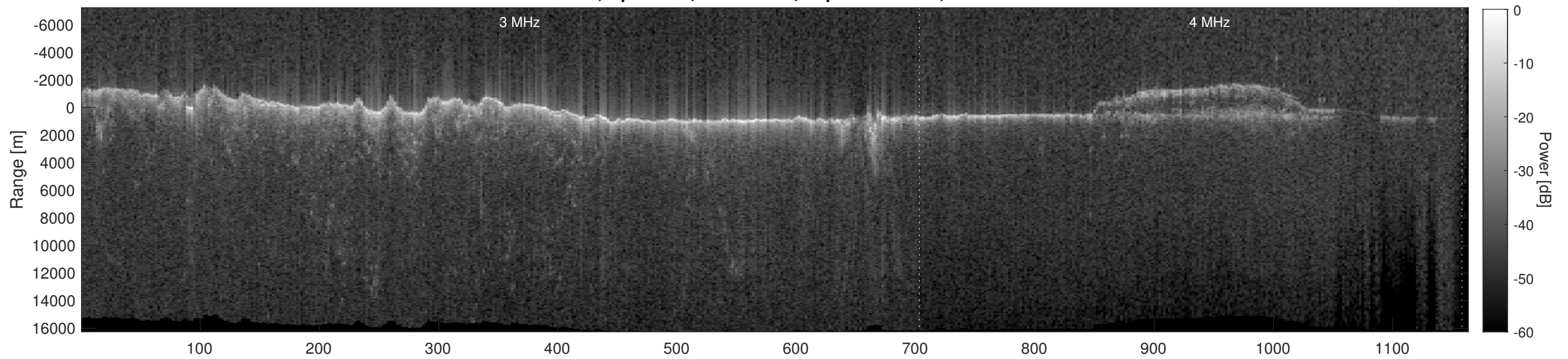
Orbit 7891, Depth-Corrected Cluttergram
