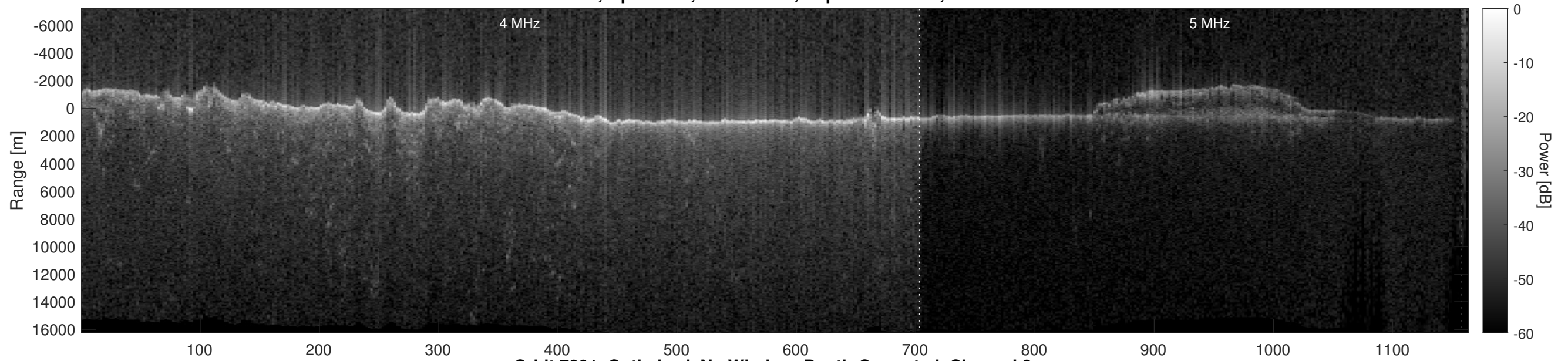
Orbit 7891, Optimized, No Window, Depth-Corrected, Channel 2
