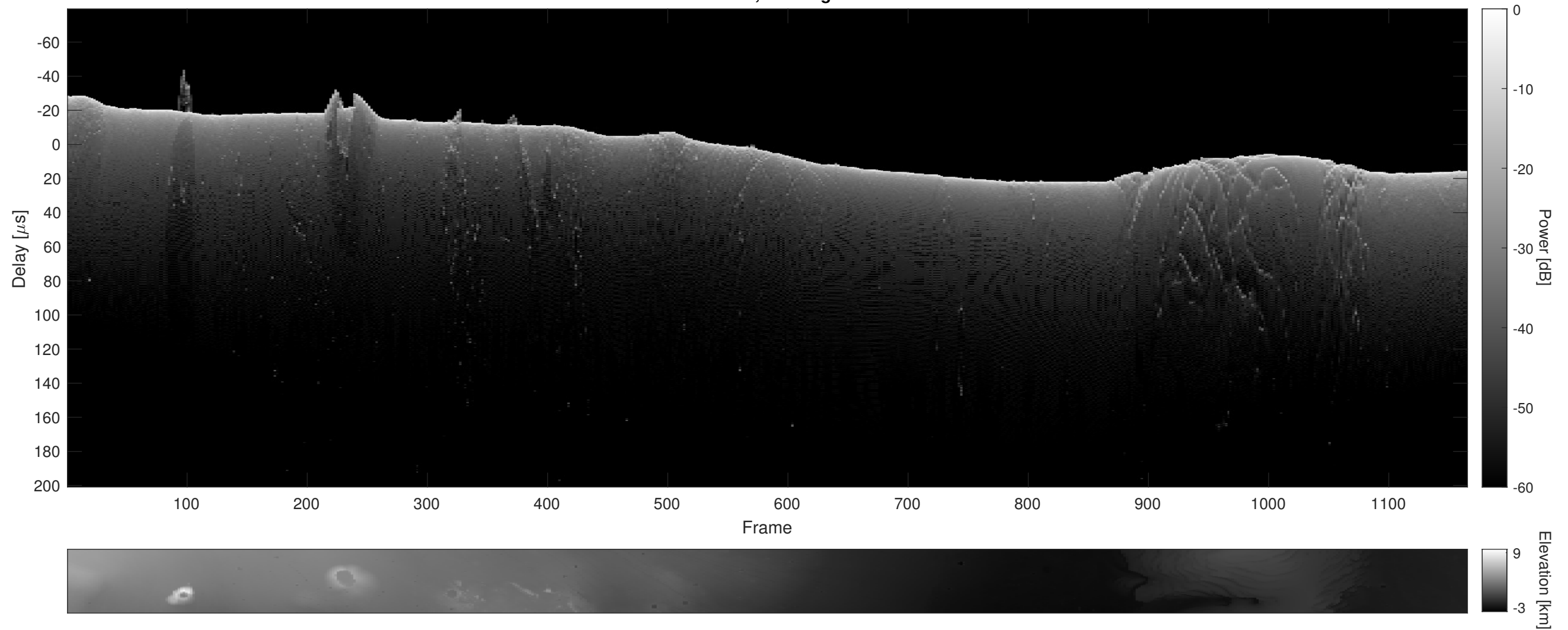
Orbit 7892, Cluttergram
