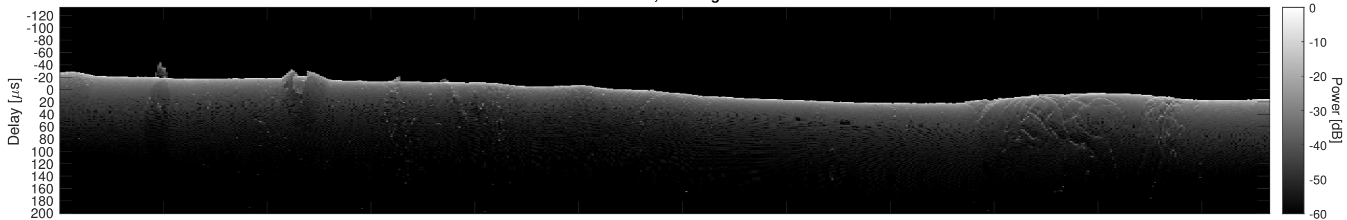
Orbit 7892, Cluttergram
