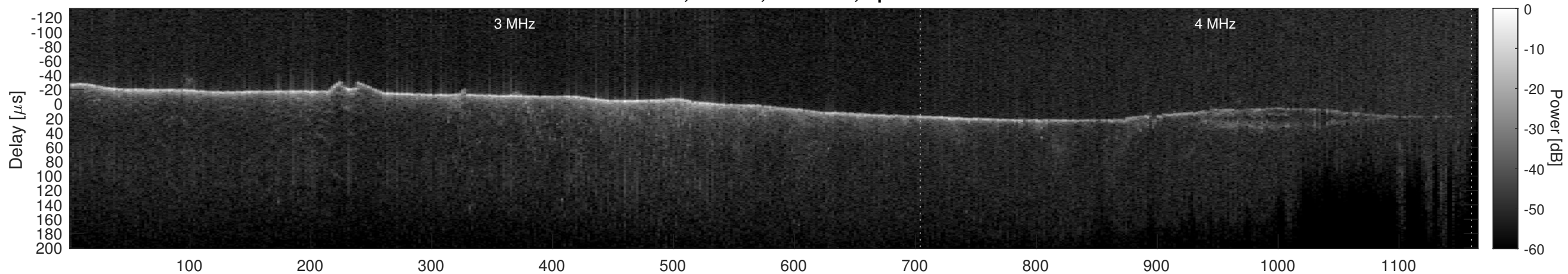
Orbit 7892, Cluttergram
