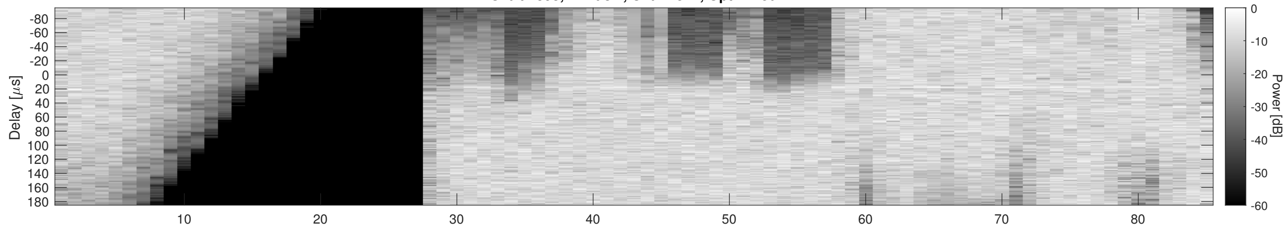
Orbit 7893, Cluttergram
