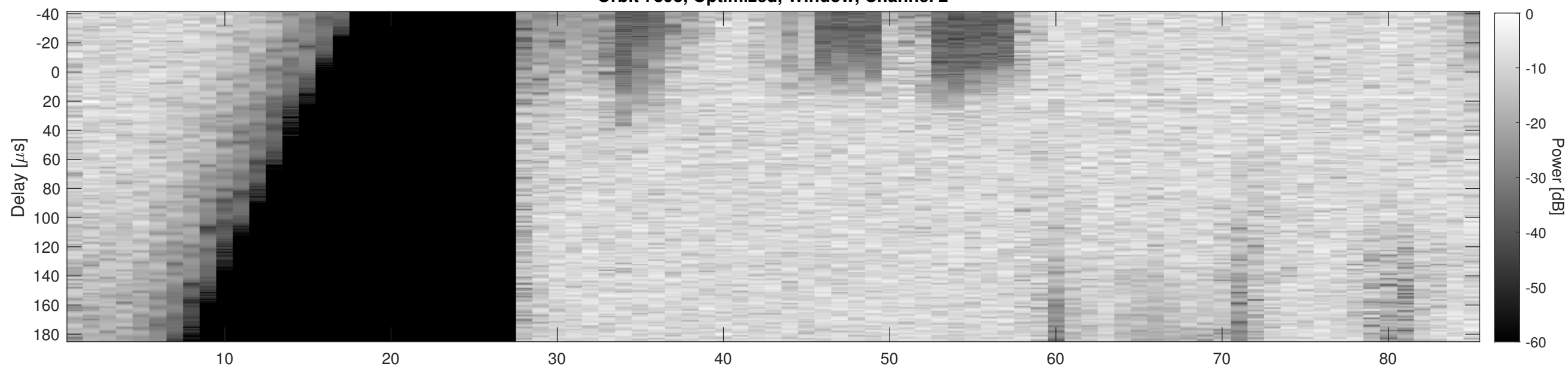
Orbit 7893, Cluttergram
