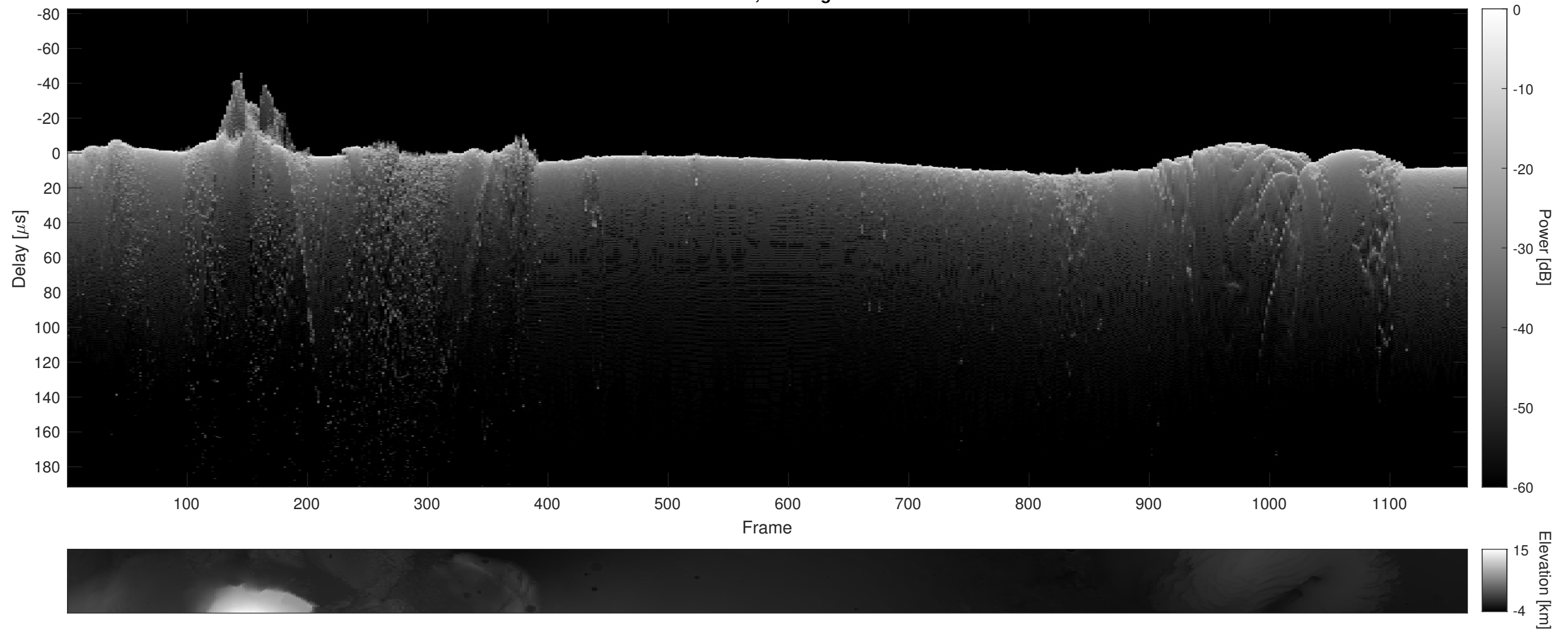
Orbit 7896, Cluttergram
