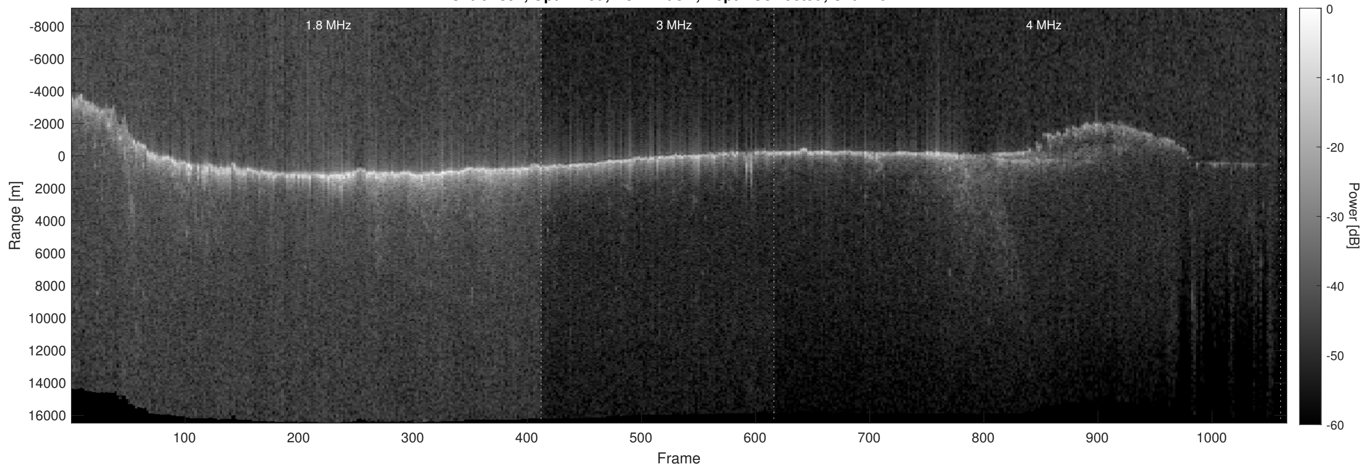
Orbit 7897, Optimized, No Window, Depth-Corrected, Channel 2
