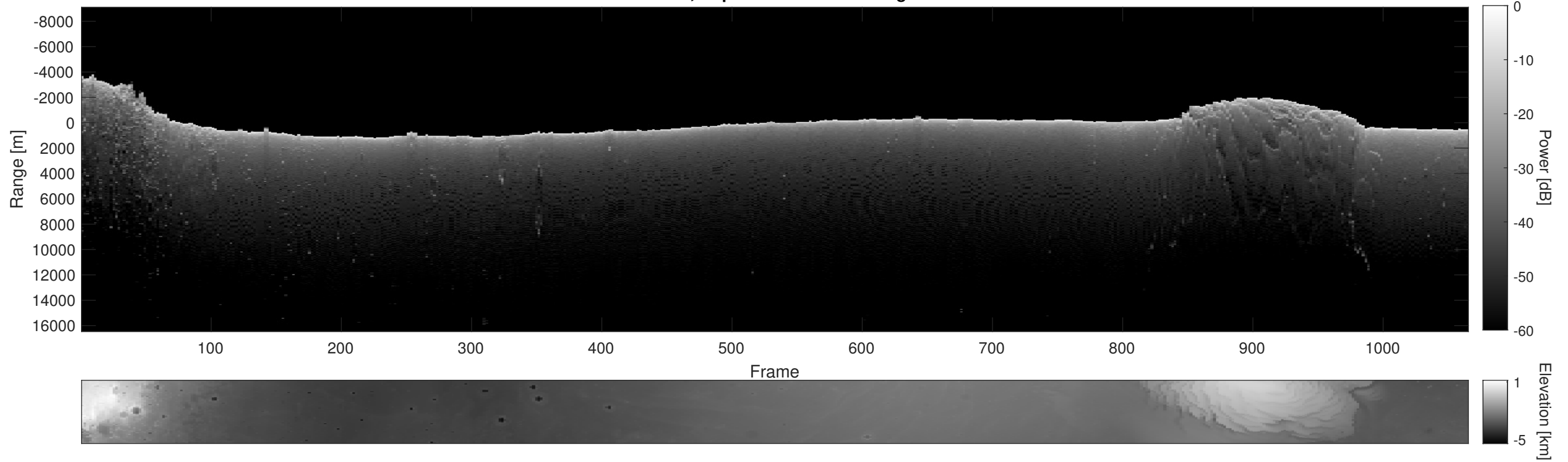
Orbit 7897, Depth-Corrected Cluttergram
