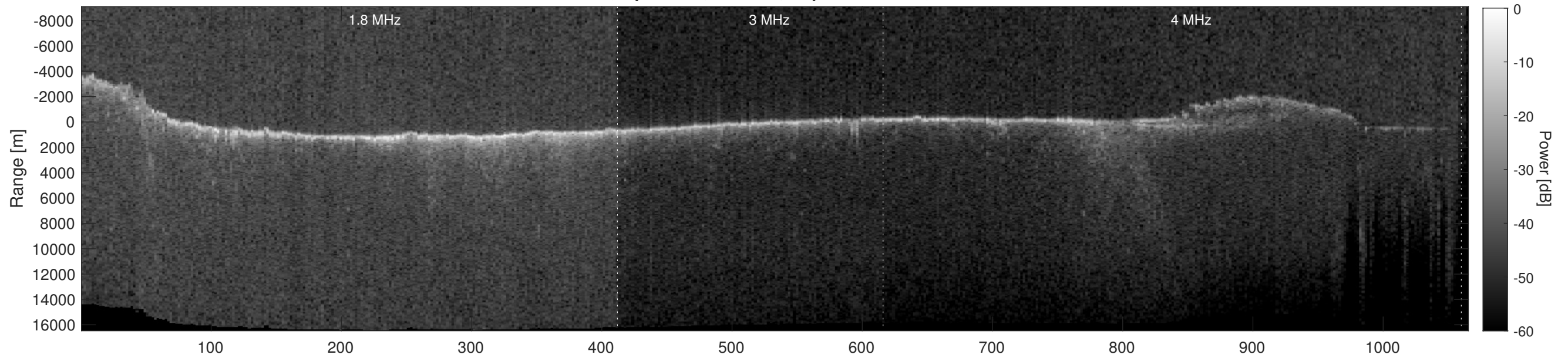
Orbit 7897, Depth-Corrected Cluttergram
