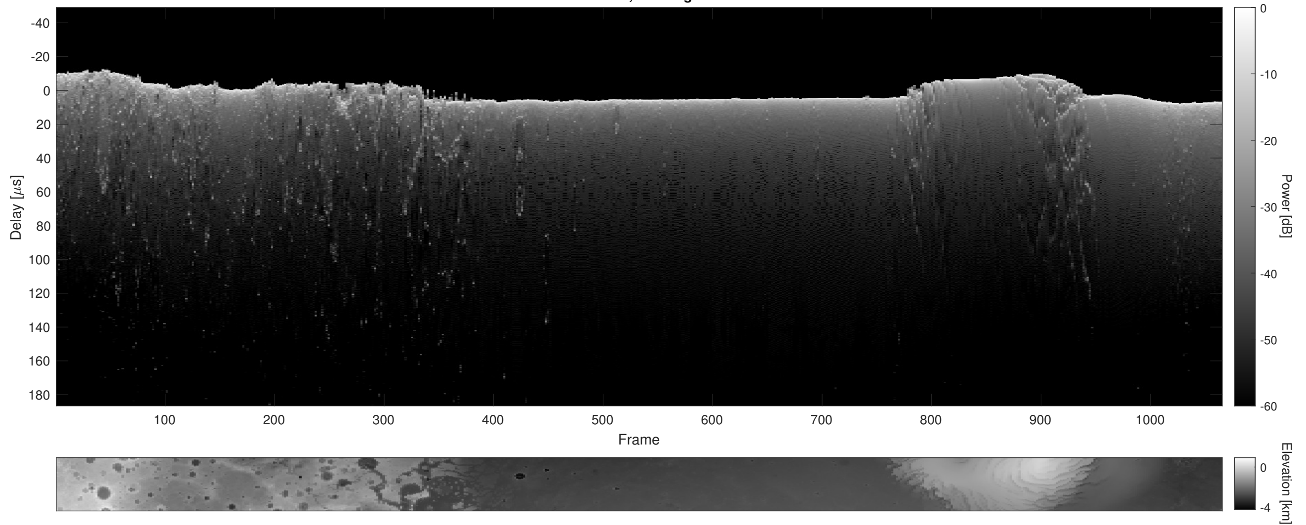
Orbit 7898, Cluttergram
