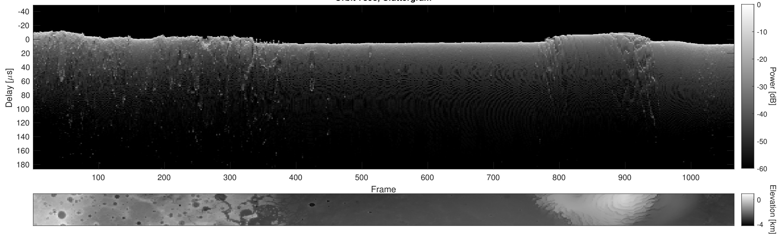
Orbit 7898, Cluttergram
