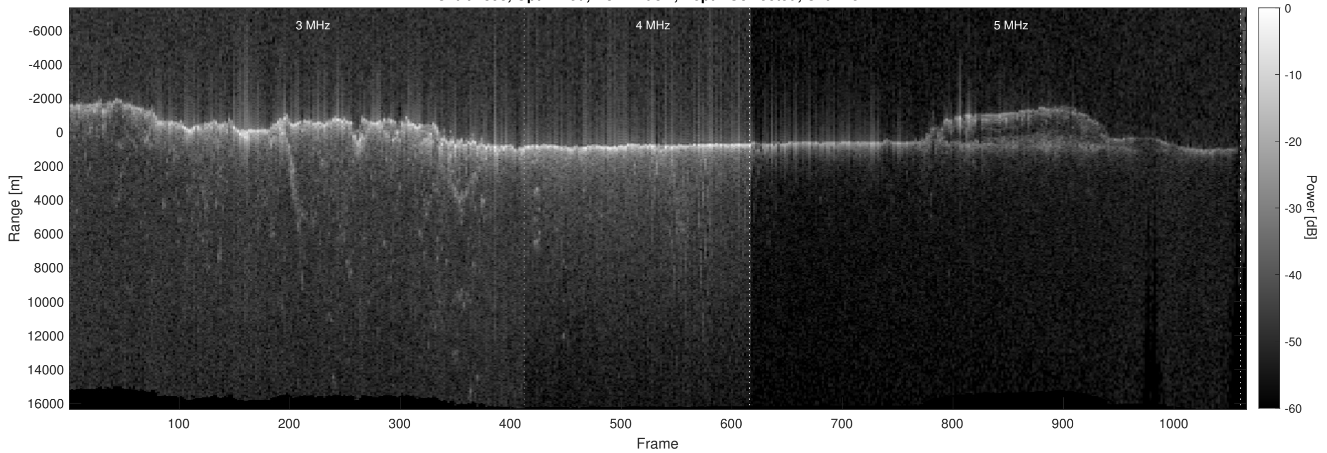
Orbit 7898, Optimized, No Window, Depth-Corrected, Channel 2
