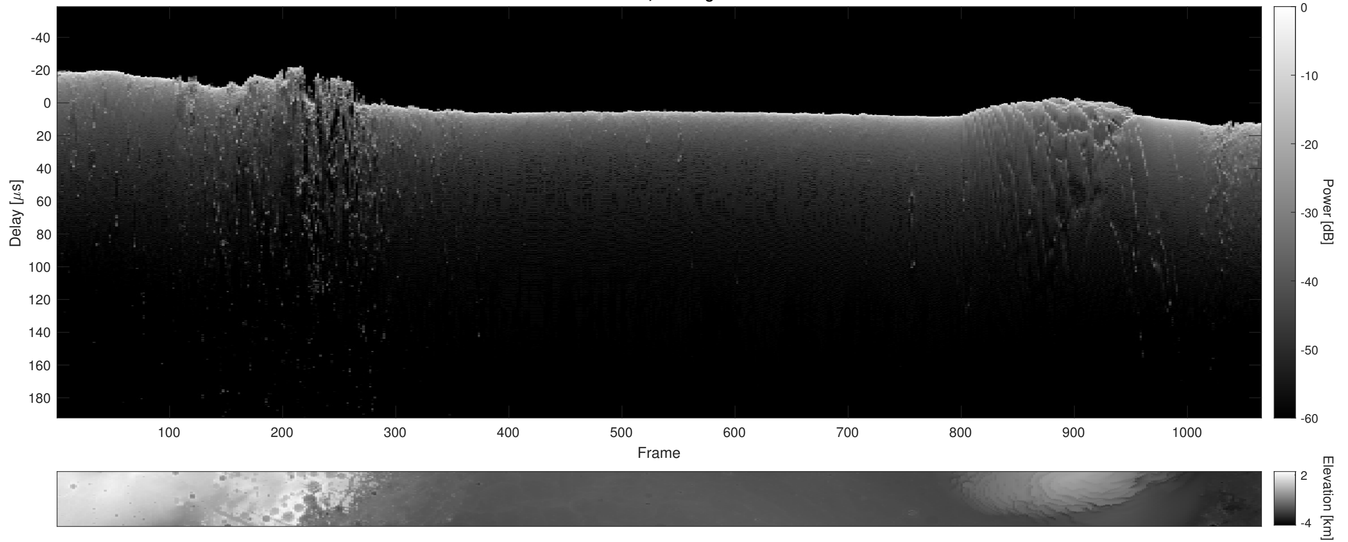
Orbit 7901, Cluttergram
