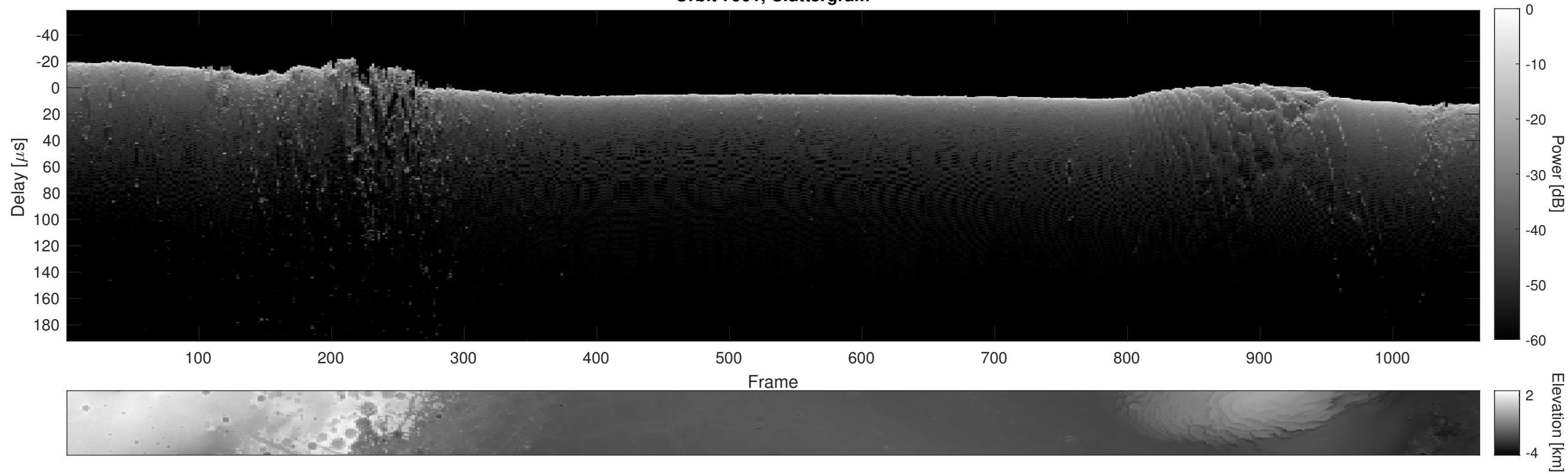
Orbit 7901, Cluttergram
