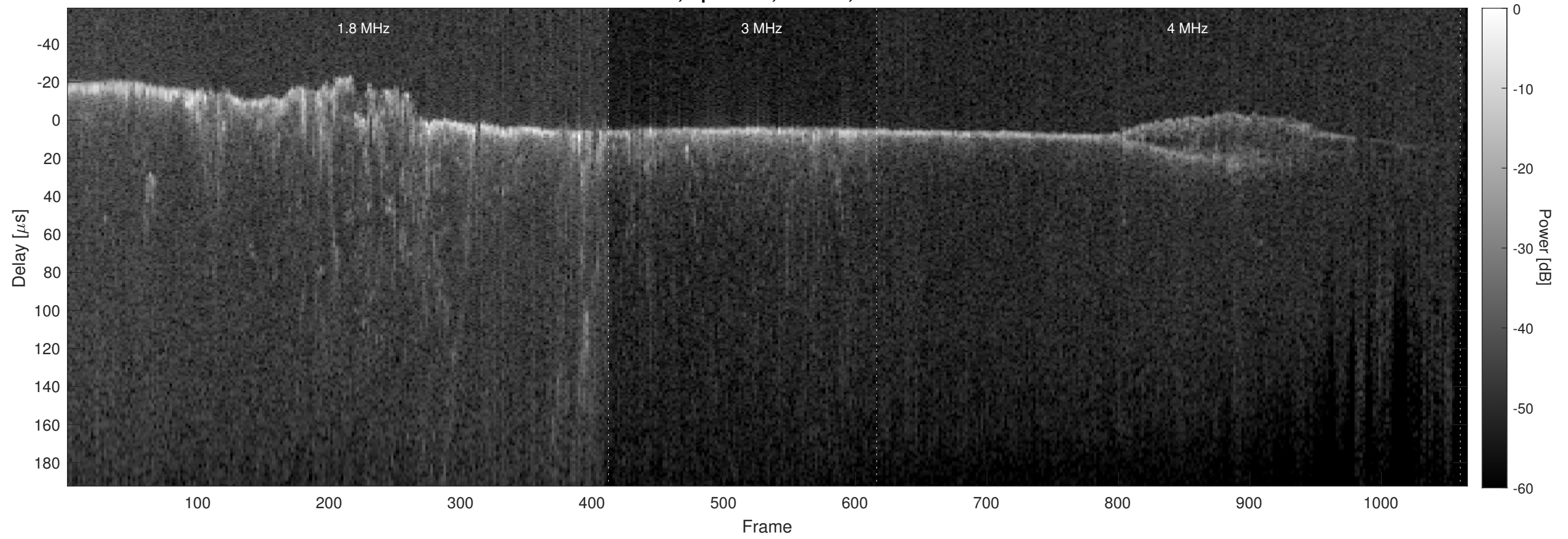
Orbit 7901, Optimized, Window, Channel 2
