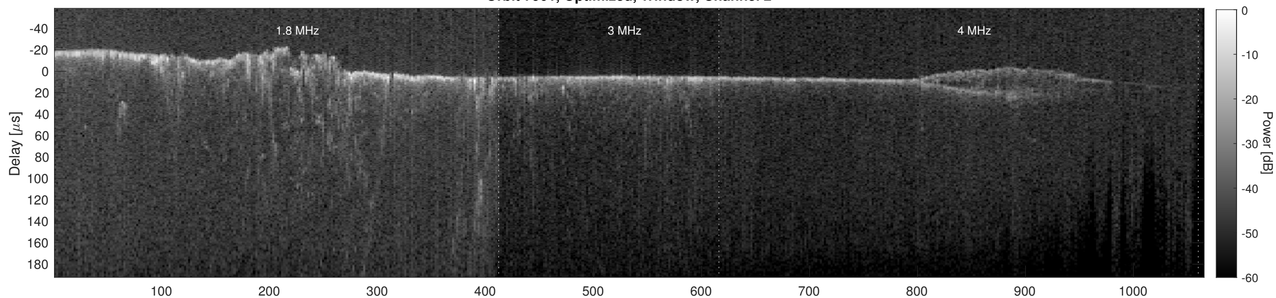
Orbit 7901, Cluttergram
