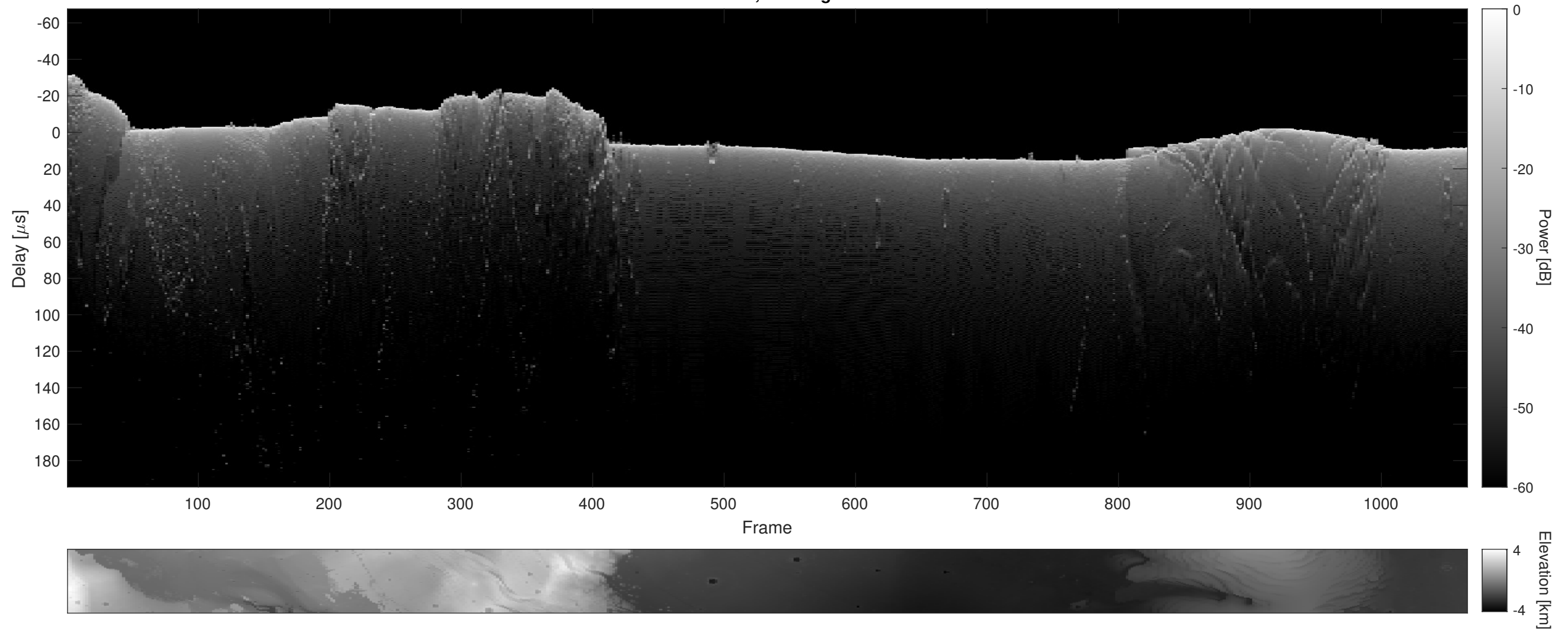
Orbit 7906, Cluttergram
