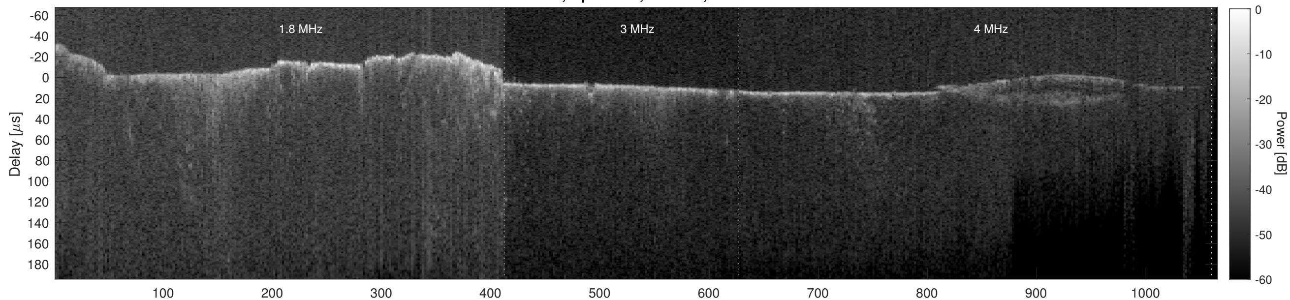
Orbit 7906, Cluttergram
