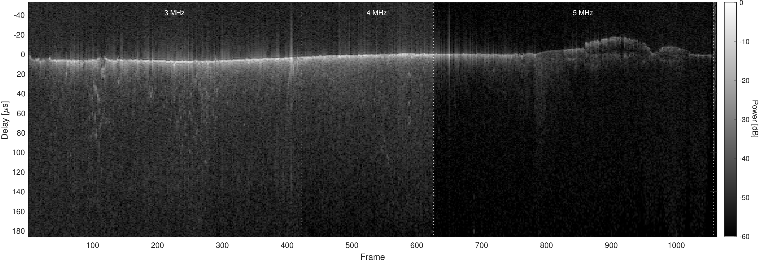
Orbit 7907, Optimized, No Window, Channel 2
