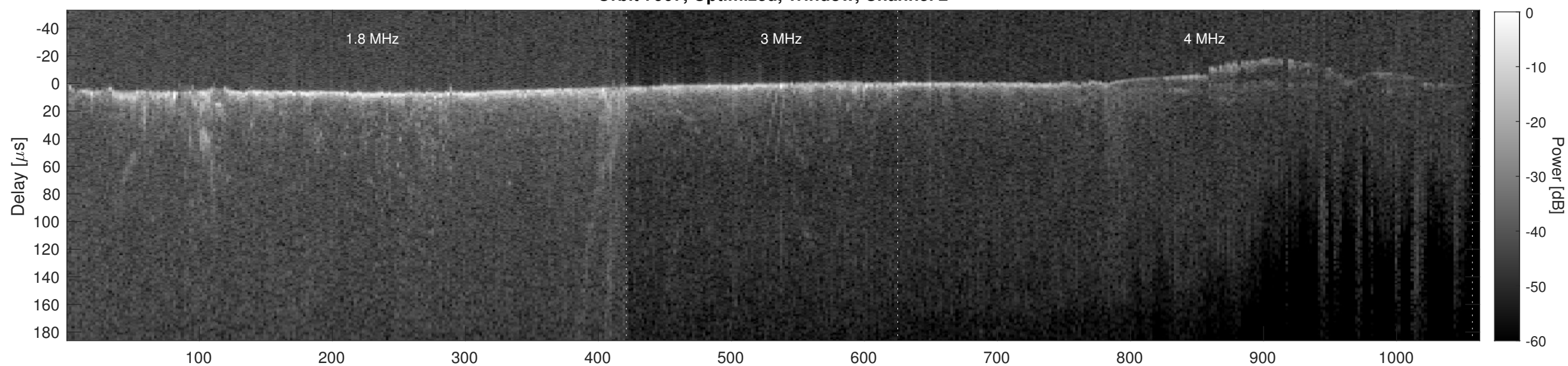
Orbit 7907, Cluttergram
