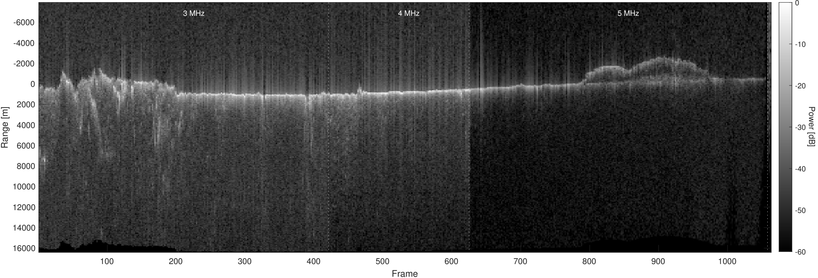
Orbit 7909, Optimized, No Window, Depth-Corrected, Channel 2
