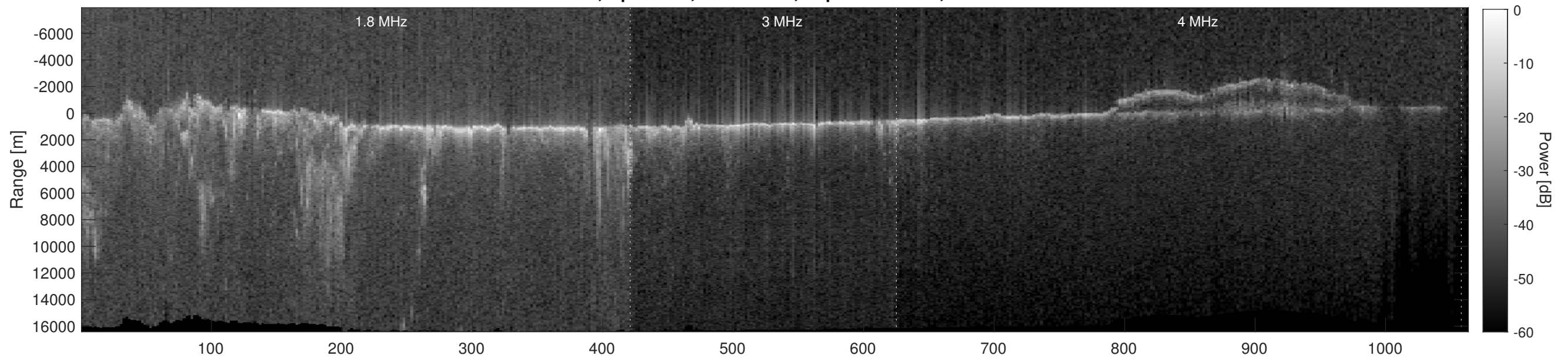
Orbit 7909, Depth-Corrected Cluttergram
