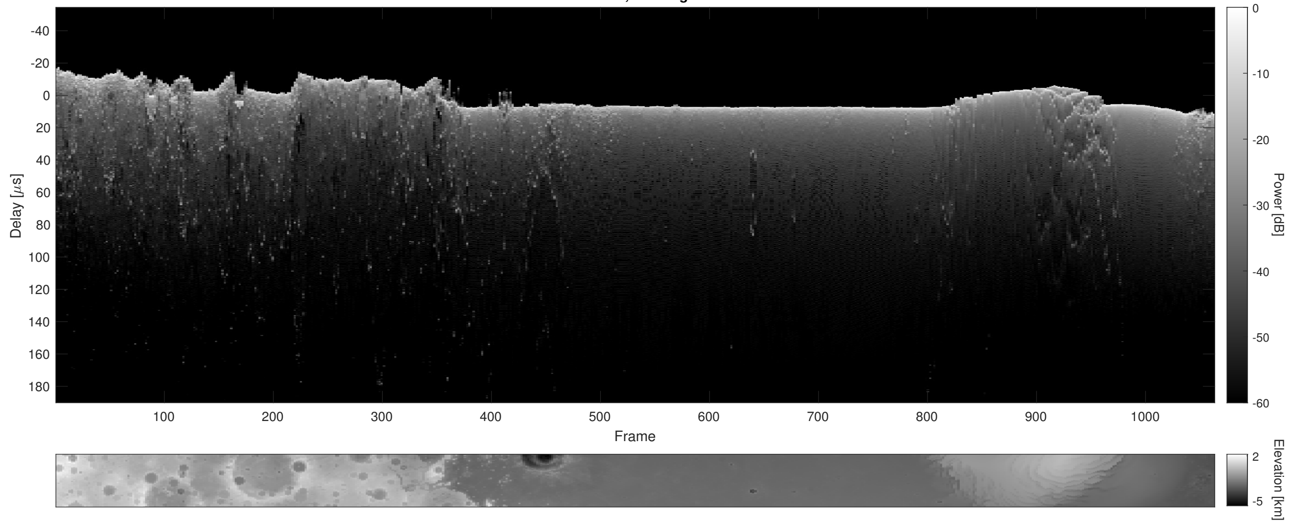
Orbit 7912, Cluttergram
