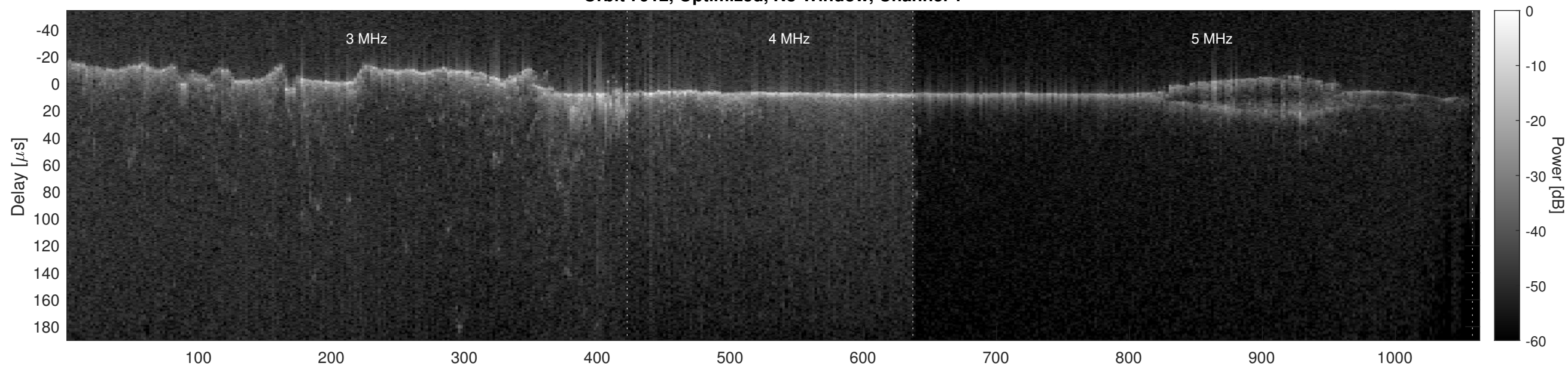
Orbit 7912, Optimized, No Window, Channel 2
