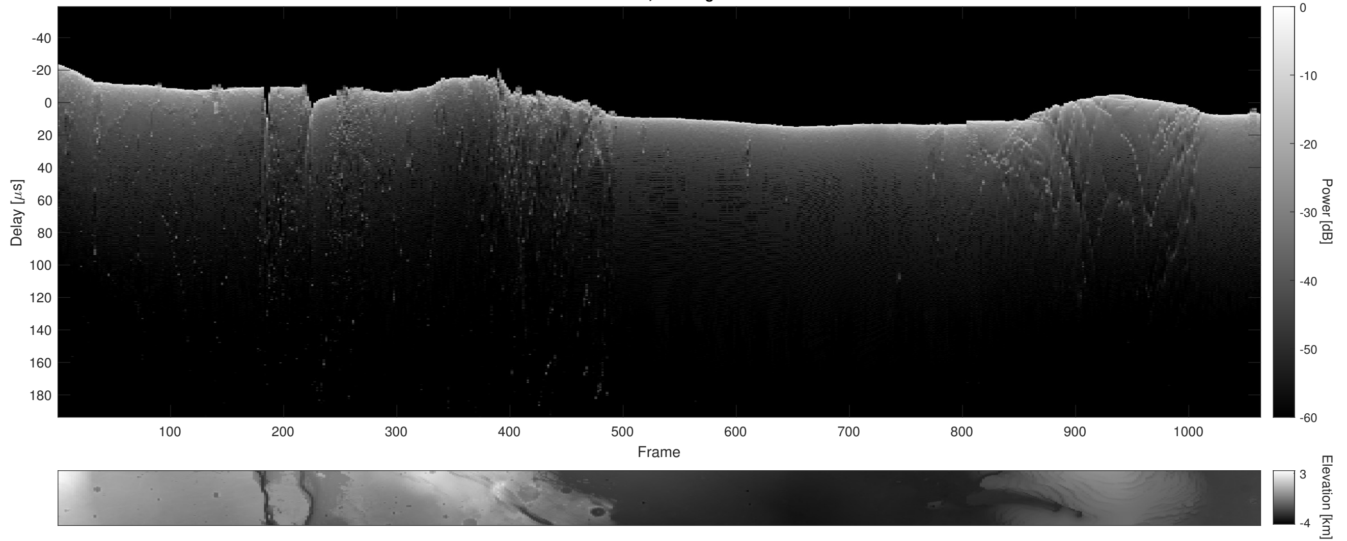
Orbit 7913, Cluttergram
