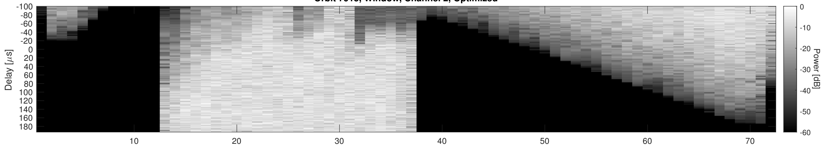
Orbit 7915, Cluttergram
