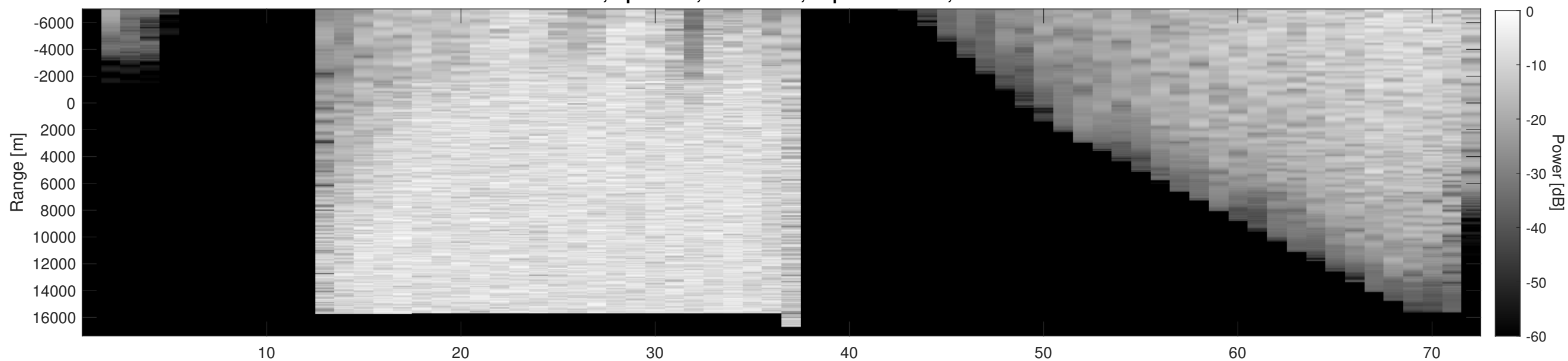
Orbit 7915, Depth-Corrected Cluttergram
