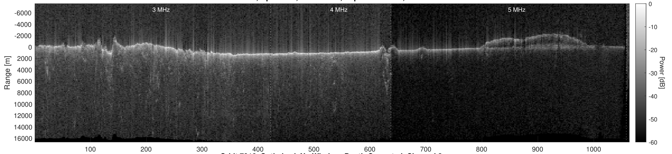
Orbit 7916, Optimized, No Window, Depth-Corrected, Channel 2
