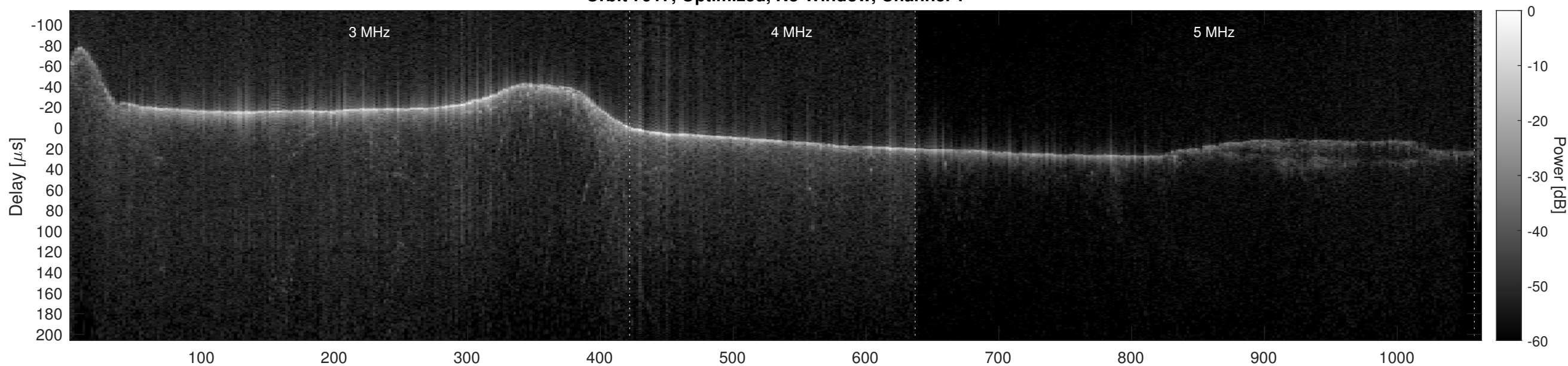
Orbit 7917, Optimized, No Window, Channel 2
