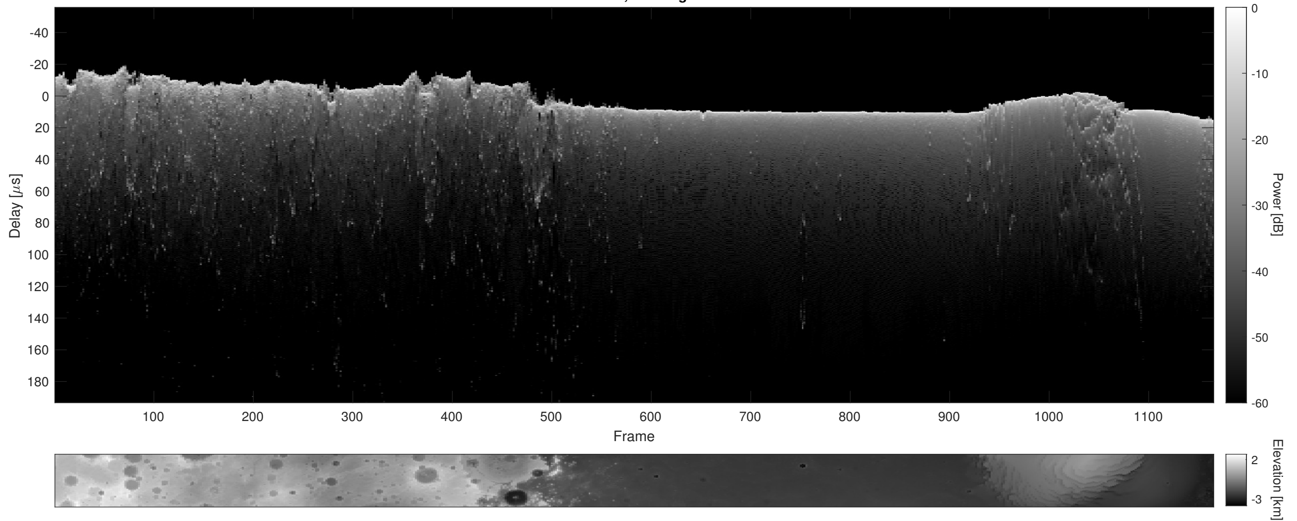
Orbit 7919, Cluttergram
