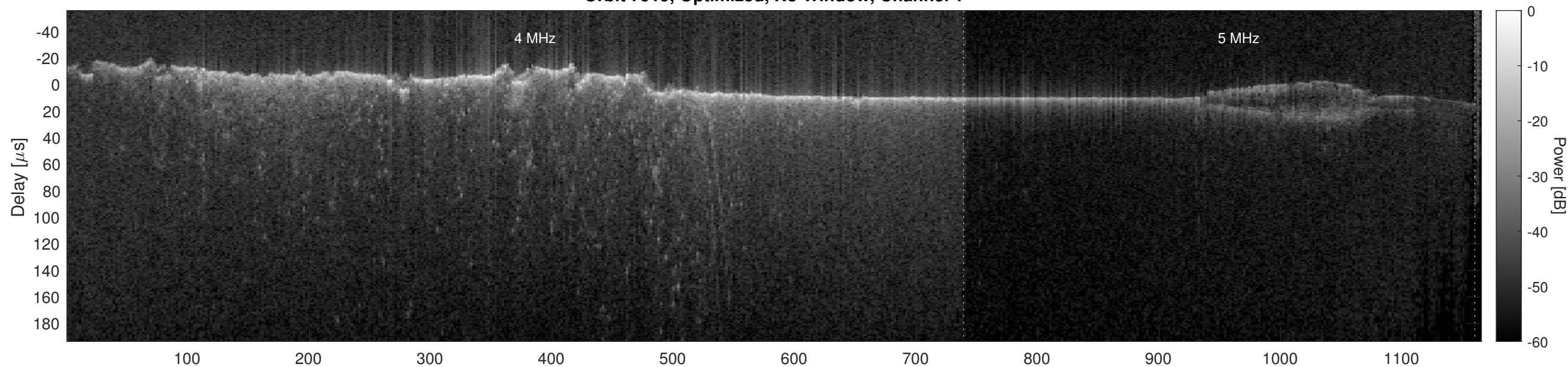
Orbit 7919, Optimized, No Window, Channel 2
