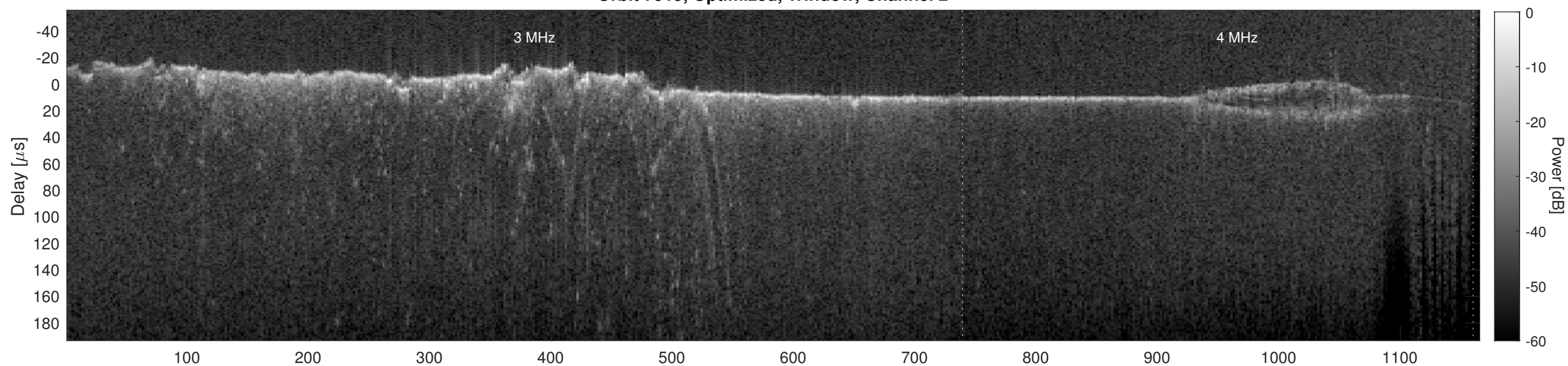
Orbit 7919, Cluttergram
