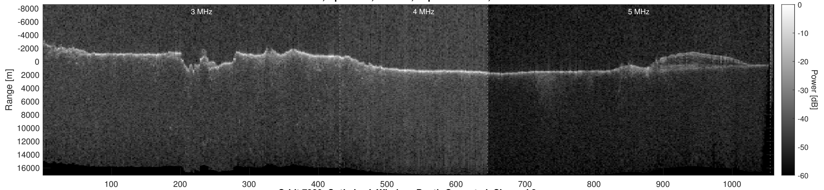
Orbit 7920, Optimized, Window, Depth-Corrected, Channel 2
