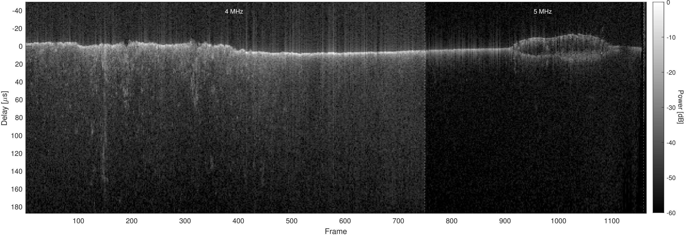
Orbit 7923, Optimized, No Window, Channel 2
